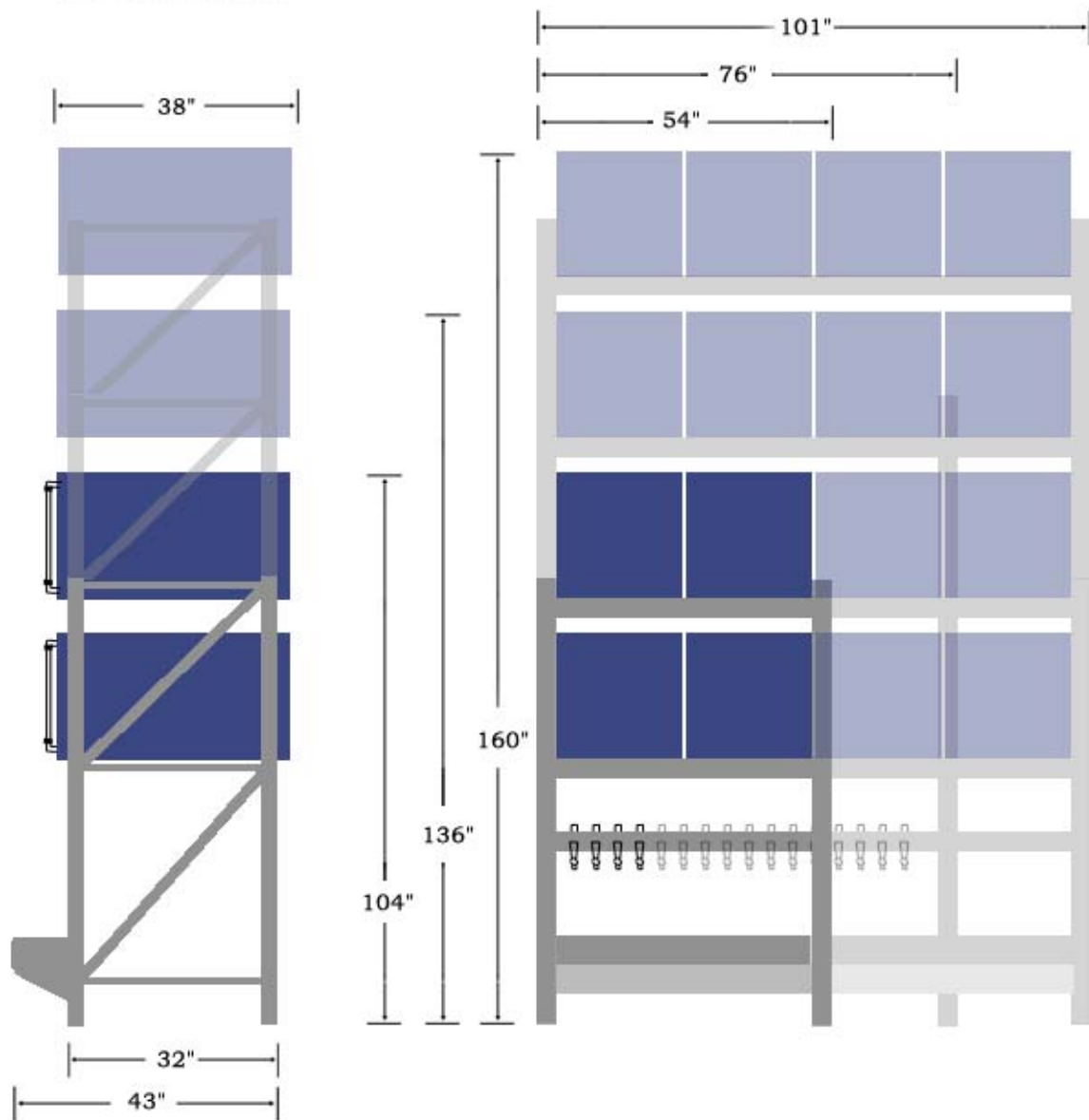
SIDE VIEW
