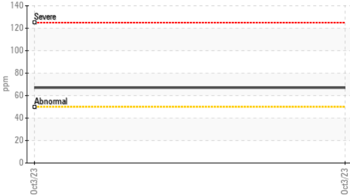
▲ Silicon (ppm)
