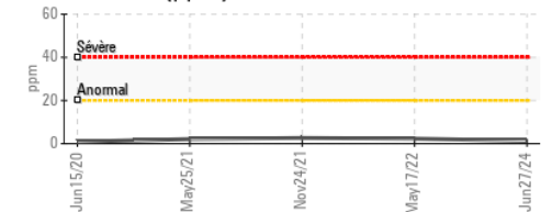
Silicium (ppm)
