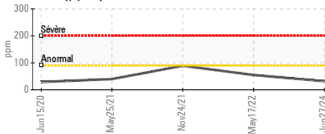
Aluminium (ppm)
