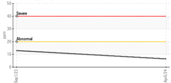
▲ Fuel Dilution
