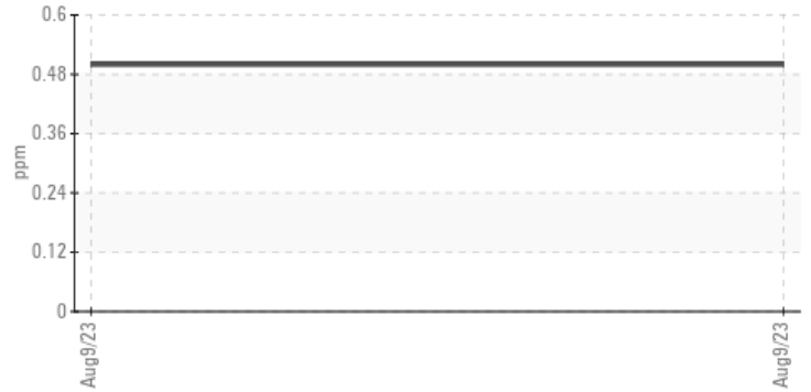
Chromium (ppm)
