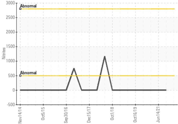
Nitrites
