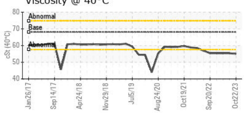
Viscosity @ 40°C
