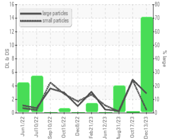
DR Ferrography
