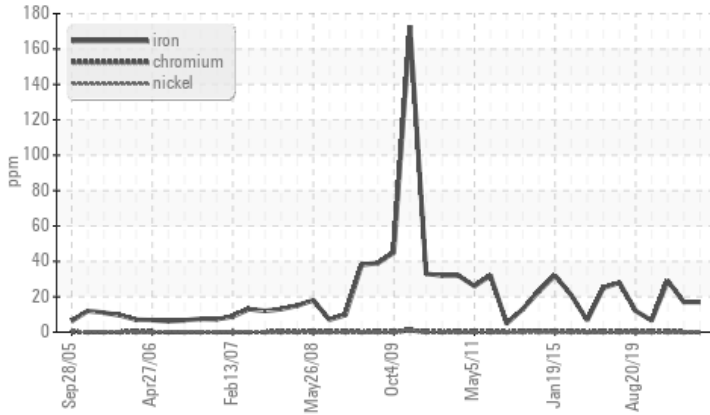
▲ Ferrous Alloys
