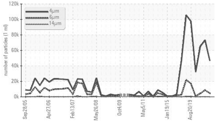
▲ Particle Trend
