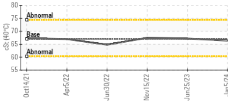
Viscosity @ 40°C
