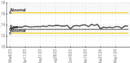
Viscosity @ 100°C
