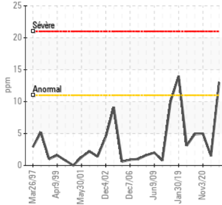
▲ Aluminium (ppm)
