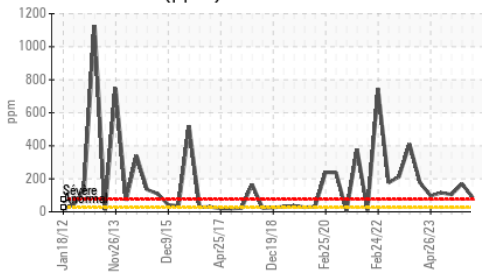
Aluminium (ppm)
