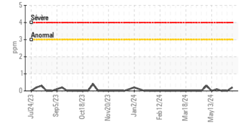
Silicium (ppm)
