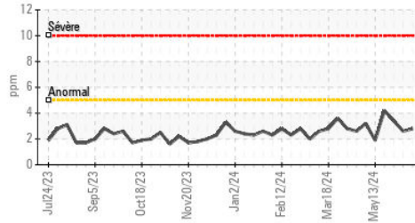
Cuivre (ppm)
