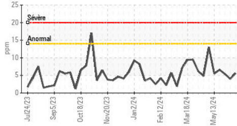
Aluminium (ppm)
