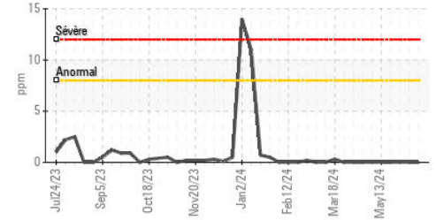
Chrome (ppm)
